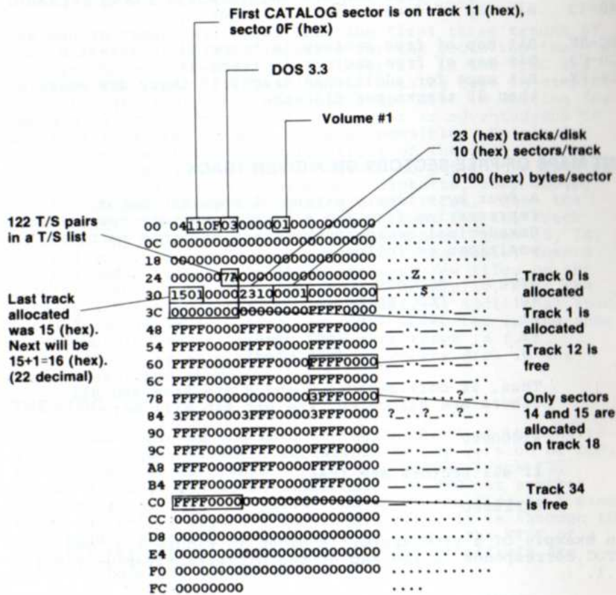
FIGURE 4.2 — EXAMPLE VTOC
