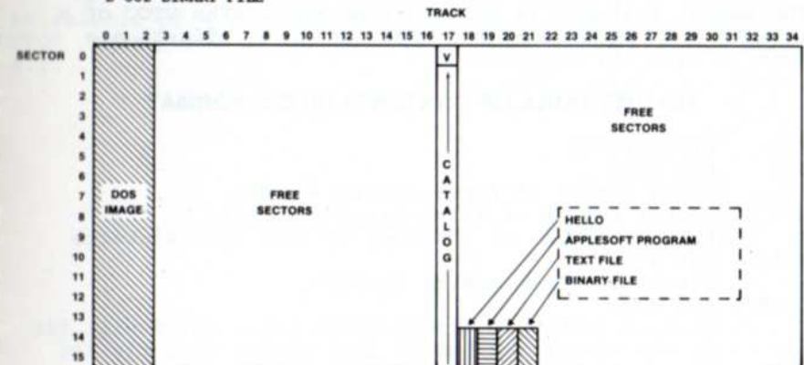
A TYPICAL 16 SECTOR DISKETTE MAP FIGURE 4.1
